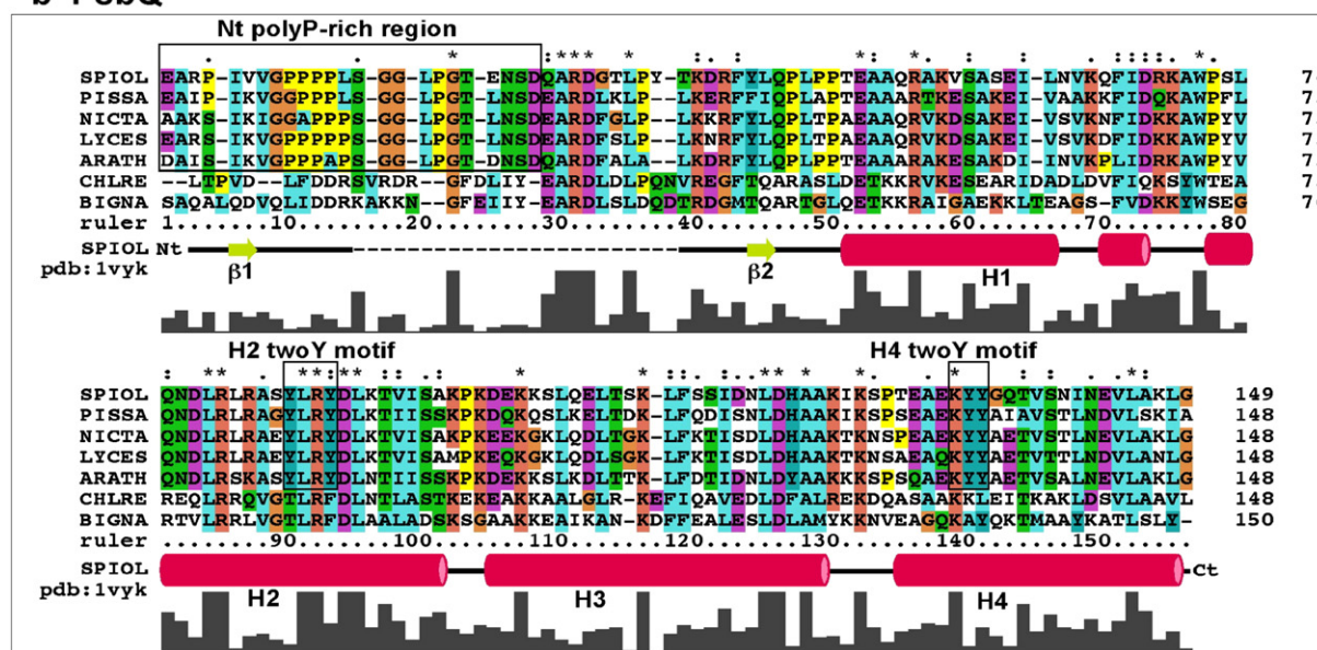
Fig. 1. MSAs of PsbP and PsbQ from 7 species (5 higher plants and 2 green algae quoted in Methods). The alignments include the known secondary structure for Nicotiana tabacum PsbP (pdb 1V2B) and Spinacea oleracea PsbQ (pdb 1VYK). Adjusted to the sequence space, the alpha-helices are drawn as purple cylinders and the beta-strands as yellow arrows. The colour code of the residues in the alignments corresponds to the standard provided by CLUSTAL. Some significant motifs are marked with boxes and labeled.
